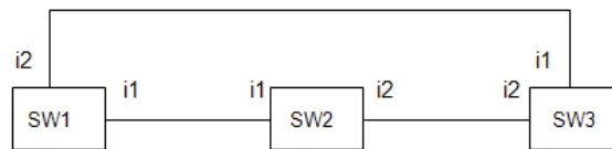
Figure 129: Determining the Root Port
