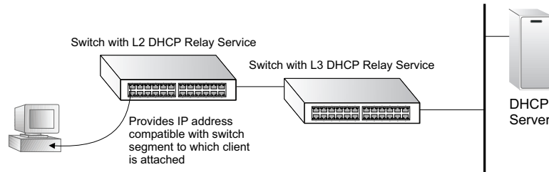
Figure 433: Layer 2 DHCP Relay Service (DHCP server on a separate network segment)
