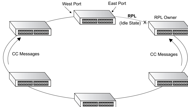
Figure 312: ERPS Ring Components
