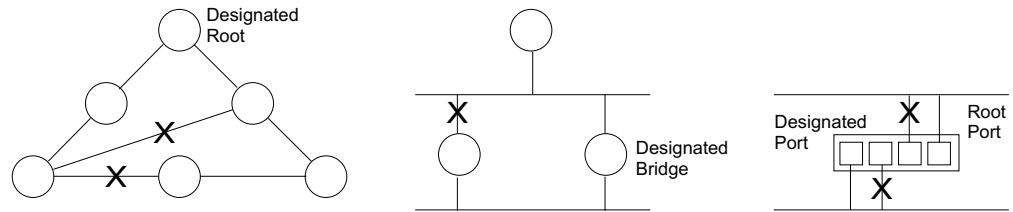
Figure 121: STP Root Ports and Designated Ports
