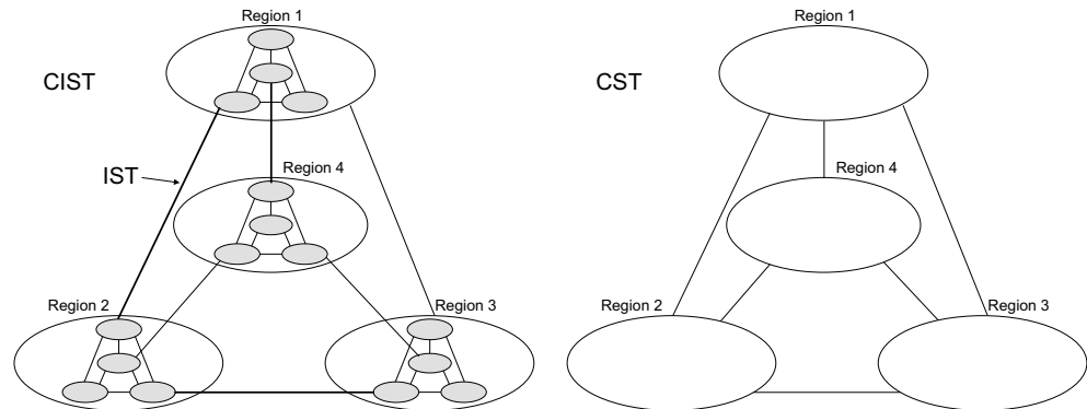
Figure 123: Spanning Tree – Common Internal, Common, Internal
