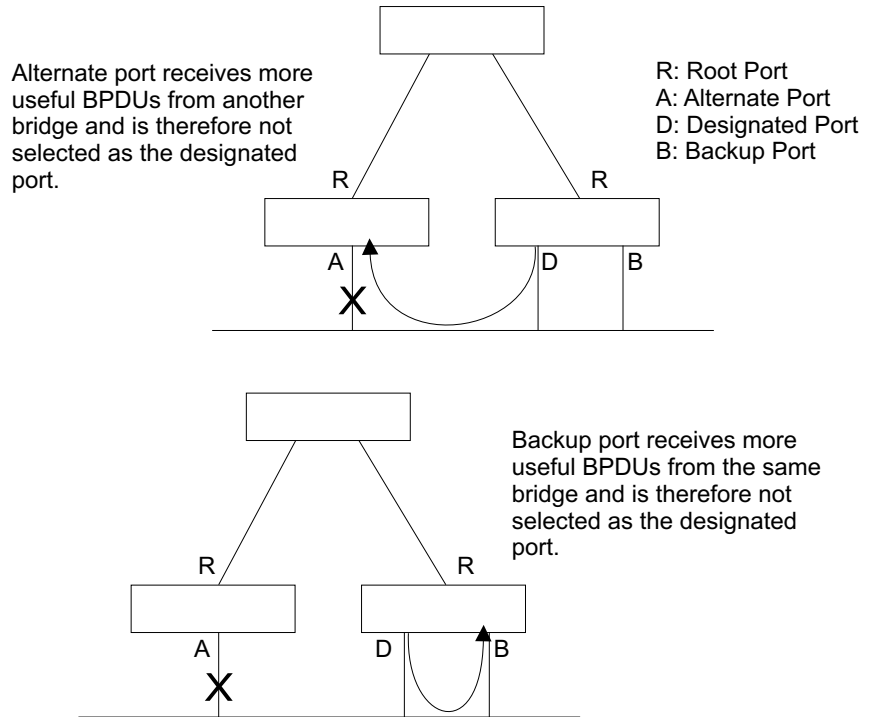
Figure 131: STA Port Roles
