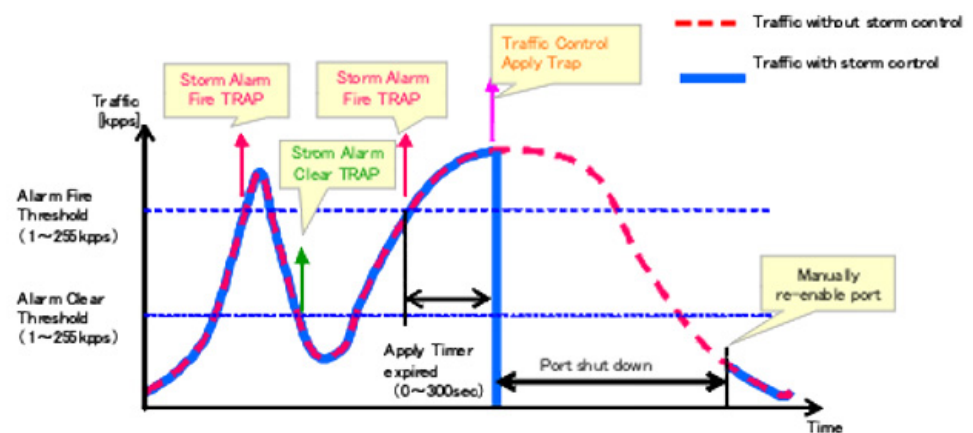
Figure 144: Storm Control by Shutting Down a Port
