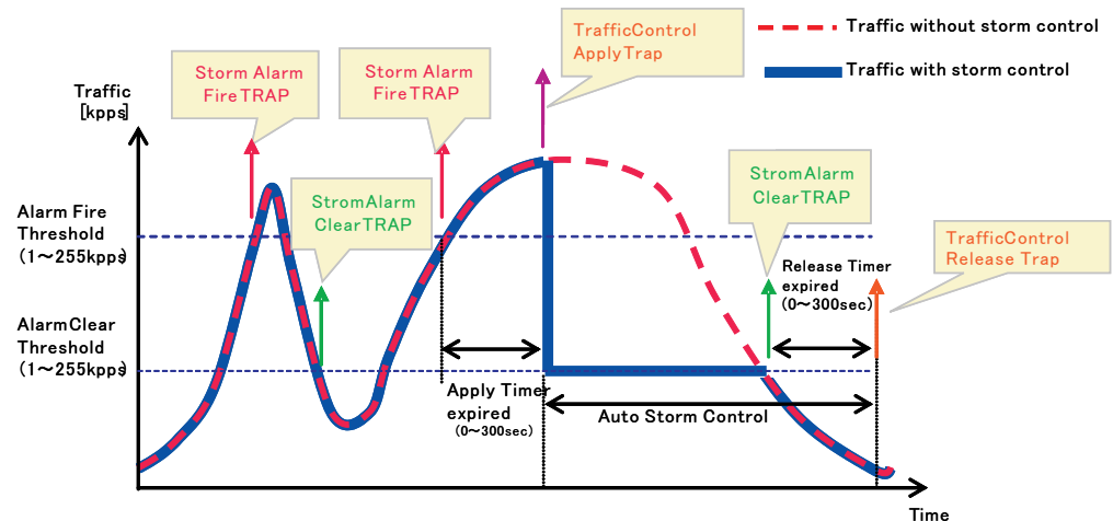
Figure 143: Storm Control by Limiting the Traffic Rate
