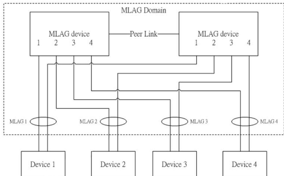
Figure 323: MLAG Domain Topology
