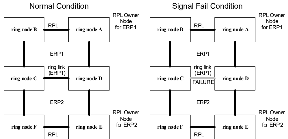
Figure 313: Ring Interconnection Architecture (Multi-ring/Ladder Network)
