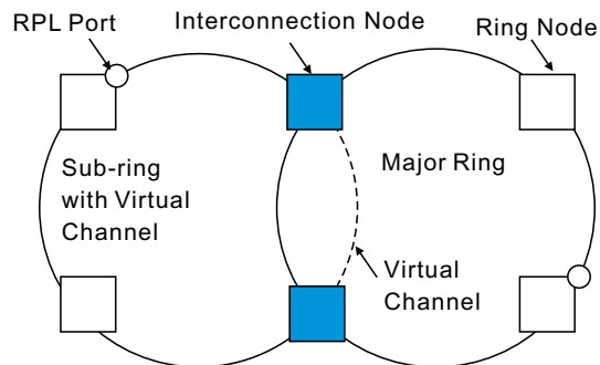
Figure 317: Sub-ring with Virtual Channel
