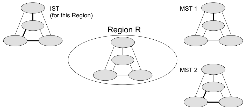
Figure 122: MSTP Region, Internal Spanning Tree, Multiple Spanning Tree
