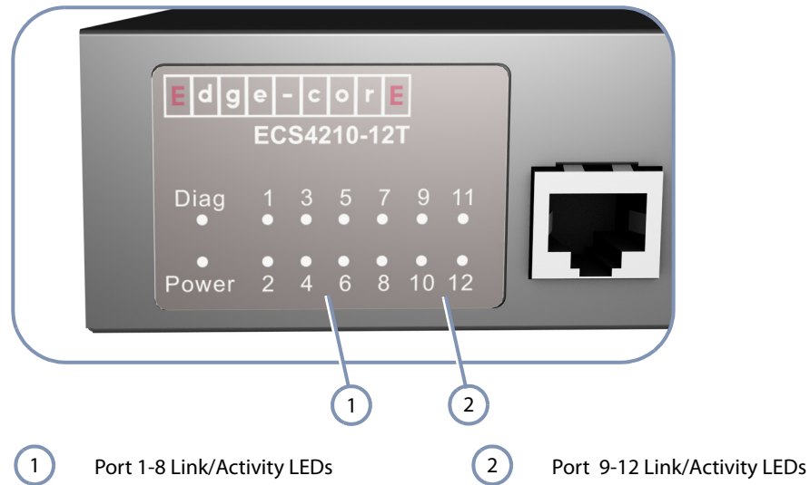
Figure 16: Port Status LEDs
