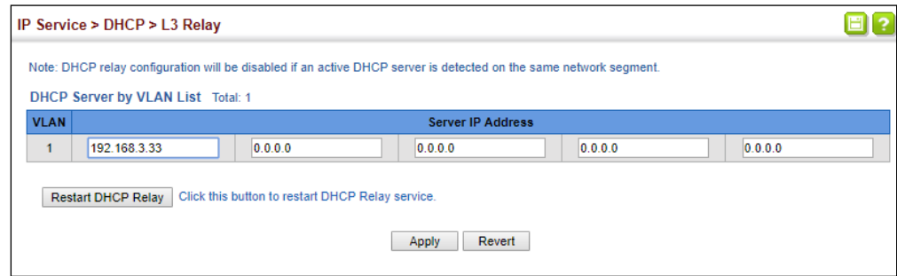
Figure 483: Configuring L3 DHCP Relay Service
