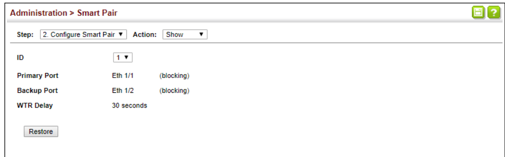
Figure 373: Displaying Port Members of a Smart Pair
