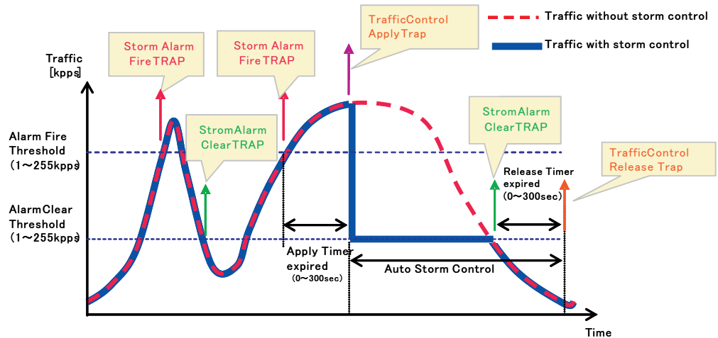
Figure 142: Storm Control by Limiting the Traffic Rate
