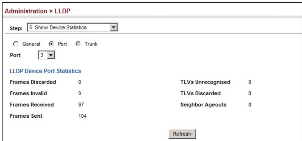
Figure 272: Displaying LLDP Device Statistics (Port)
