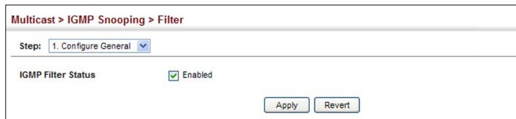
Figure 389: Enabling IGMP Filtering and Throttling
