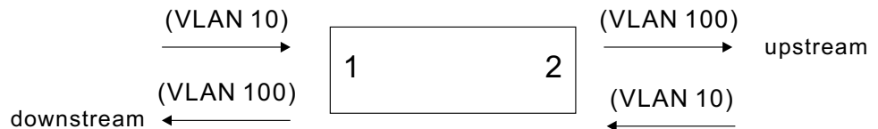
Figure 107: Configuring VLAN Translation
