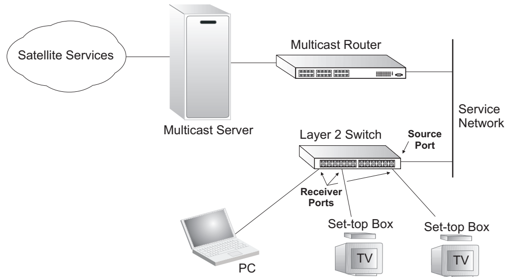
Figure 407: MVR Concept
