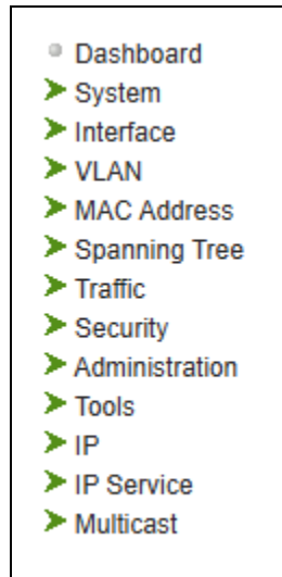
Figure 4: Main Menu
