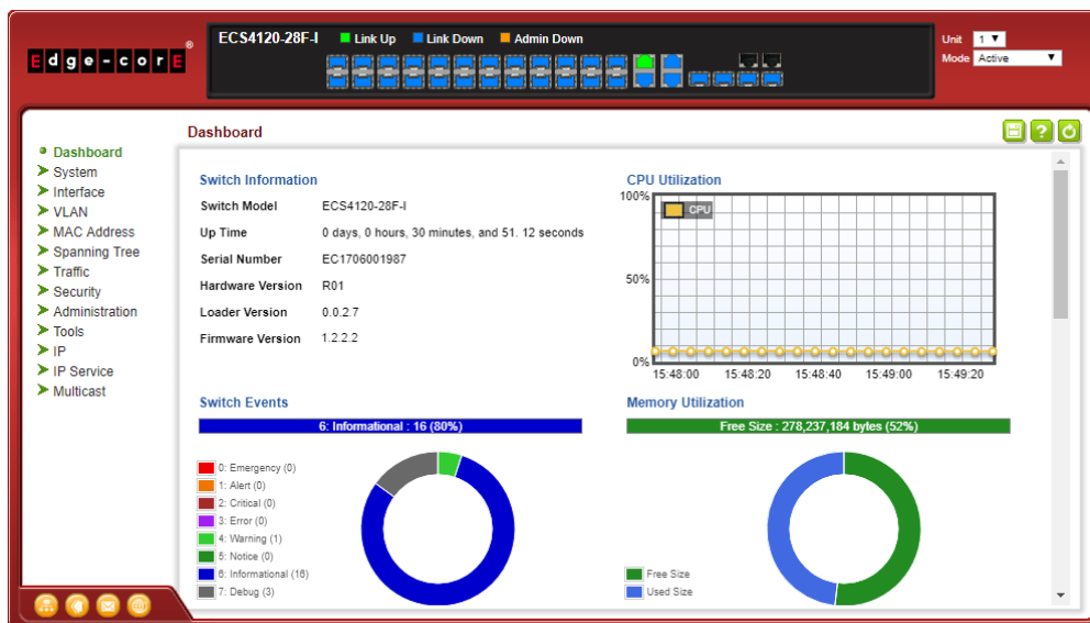
Figure 2: Home Page
