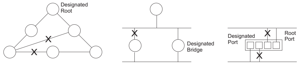
Figure 118: STP Root Ports and Designated Ports
