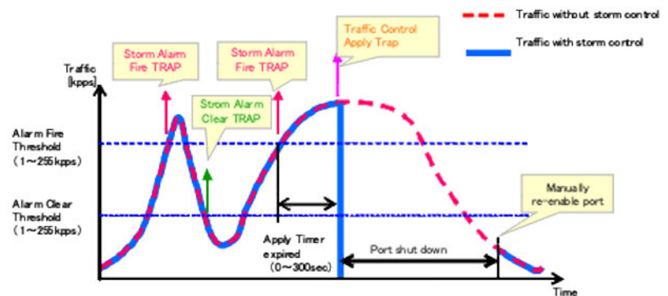
Figure 141: Storm Control by Shutting Down a Port
