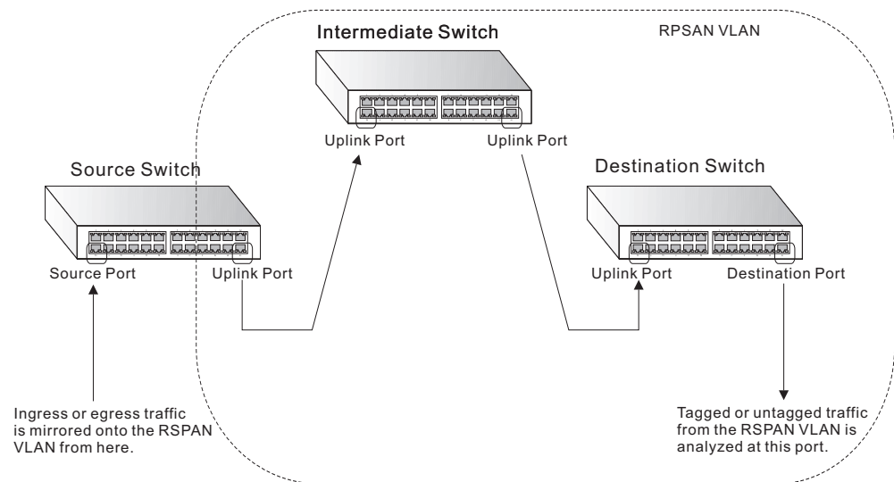
Figure 67: Configuring Remote Port Mirroring
