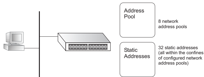
Figure 473: DHCP Server
