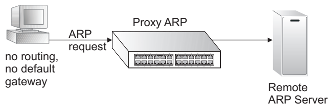
Figure 436: Proxy ARP
