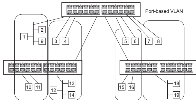
Figure 81: Using GVRP
