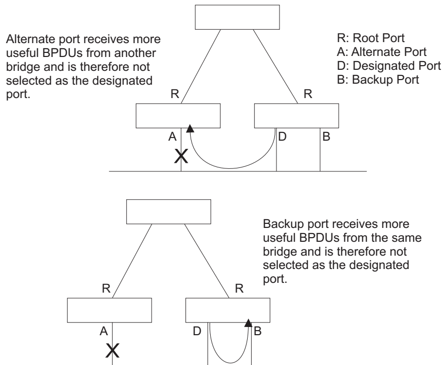
Figure 128: STA Port Roles
