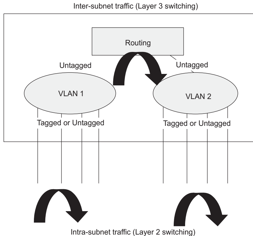
Figure 455: Virtual Interfaces and Layer 3 Routing
