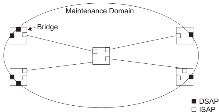
Figure 332: Single CFM Maintenance Domain
