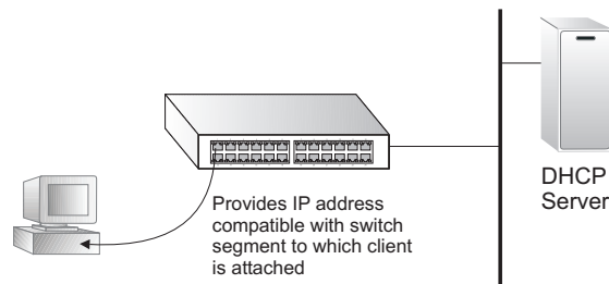
Figure 471: Layer 2 DHCP Relay Service
