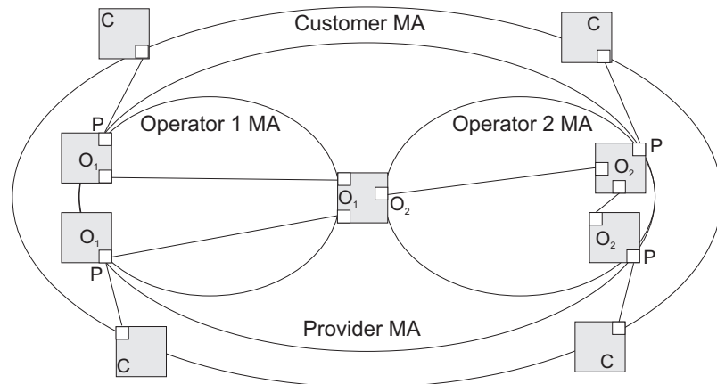
Figure 333: Multiple CFM Maintenance Domains
