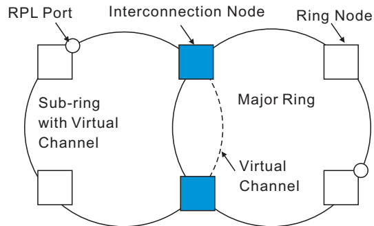
Figure 326: Sub-ring with Virtual Channel
