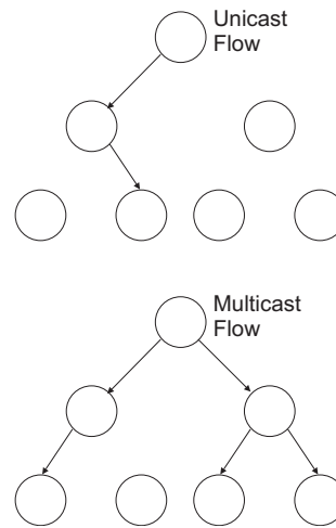
Figure 372: Multicast Filtering Concept
