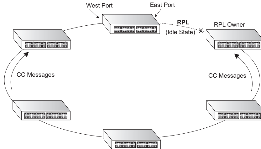
Figure 321: ERPS Ring Components
