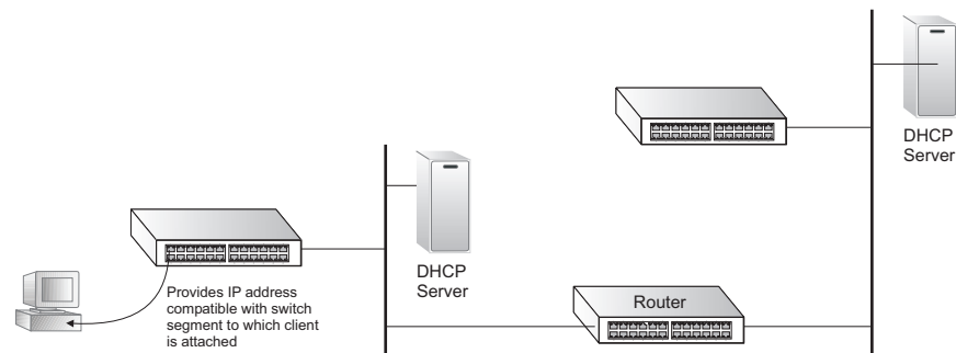
Figure 469: Layer 3 DHCP Relay Service
