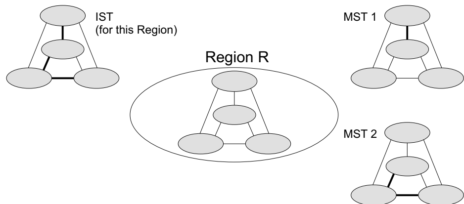
Figure 120: MSTP Region, Internal Spanning Tree, Multiple Spanning Tree
