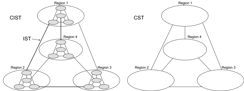
Figure 121: Spanning Tree – Common Internal, Common, Internal
