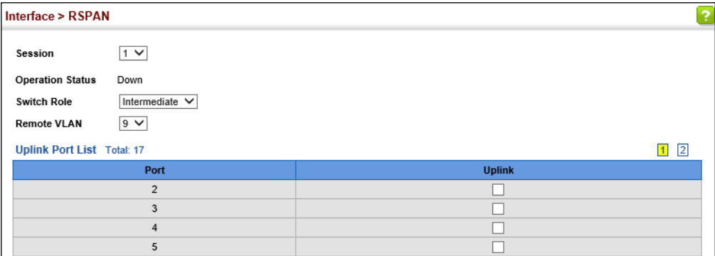
Figure 68: Configuring Remote Port Mirroring (Intermediate)
