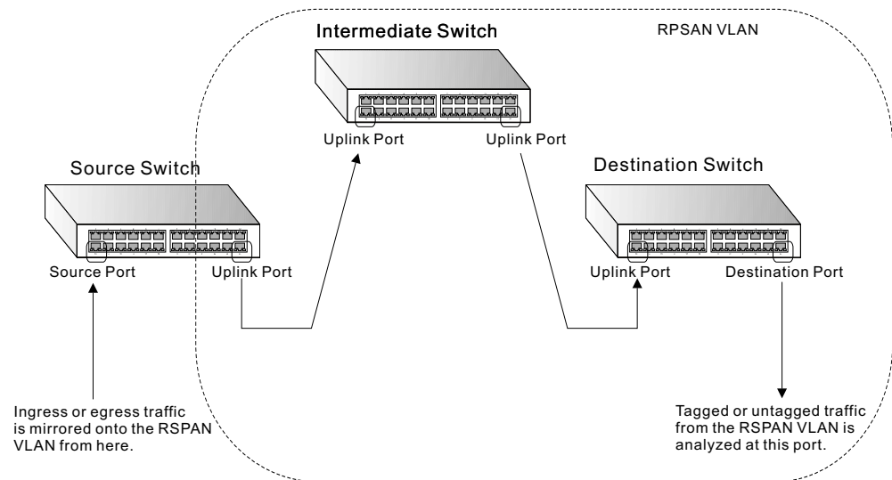
Figure 66: Configuring Remote Port Mirroring
