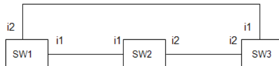
Figure 127: Determining the Root Port
