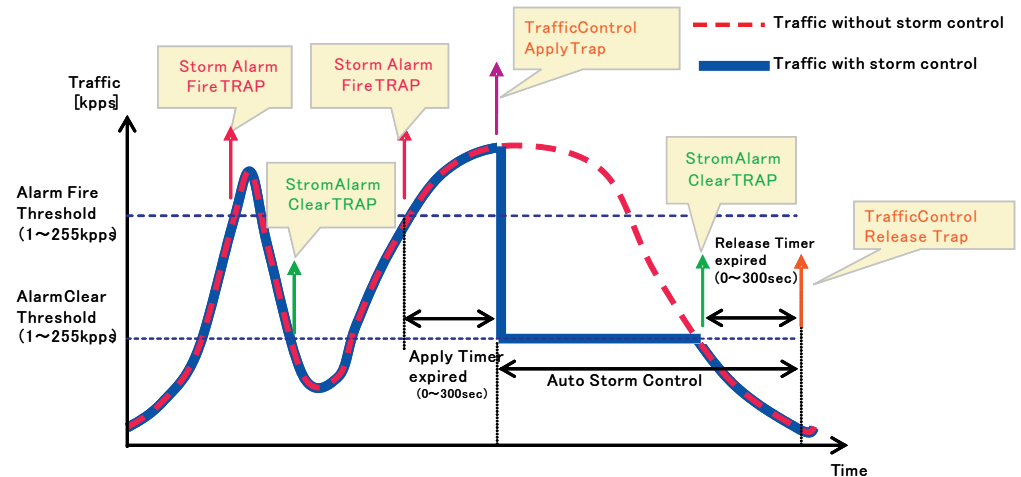
Figure 141: Storm Control by Limiting the Traffic Rate
