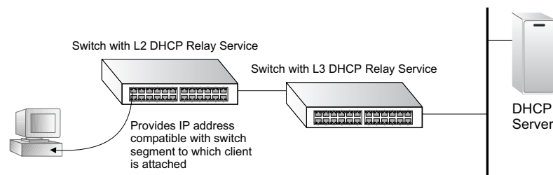
Figure 460: Layer 2 DHCP Relay Service (DHCP server on a separate network segment)
