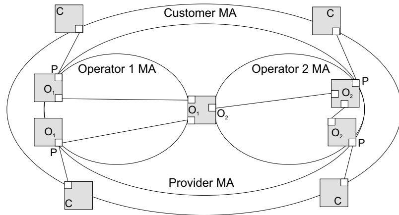
Figure 317: Multiple CFM Maintenance Domains
