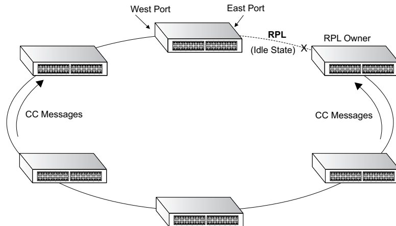
Figure 305: ERPS Ring Components
