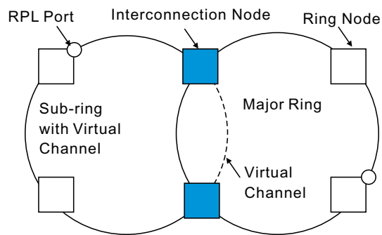
Figure 310: Sub-ring with Virtual Channel
