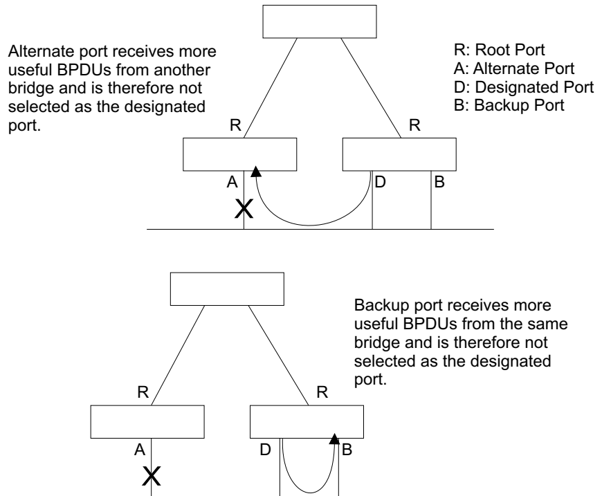
Figure 129: STA Port Roles
