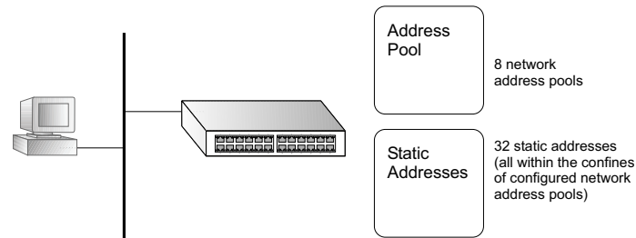
Figure 491: DHCP Server
