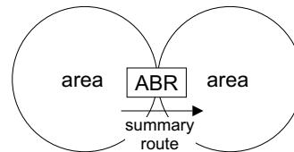
Figure 549: Route Summarization for ABRs
