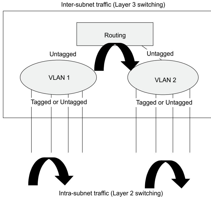
Figure 510: Virtual Interfaces and Layer 3 Routing
