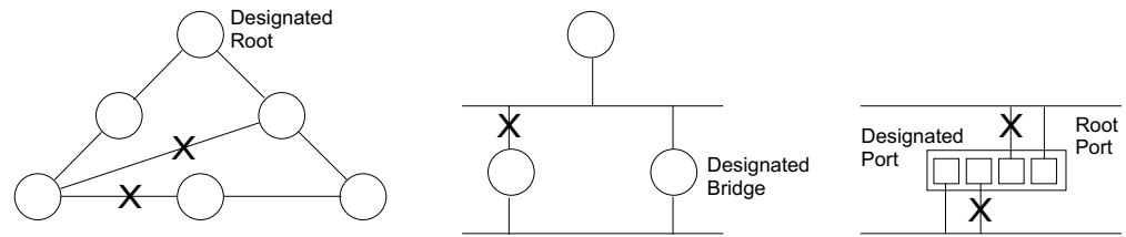
Figure 124: STP Root Ports and Designated Ports
