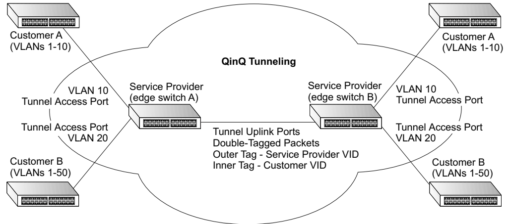
Figure 94: QinQ Operational Concept
