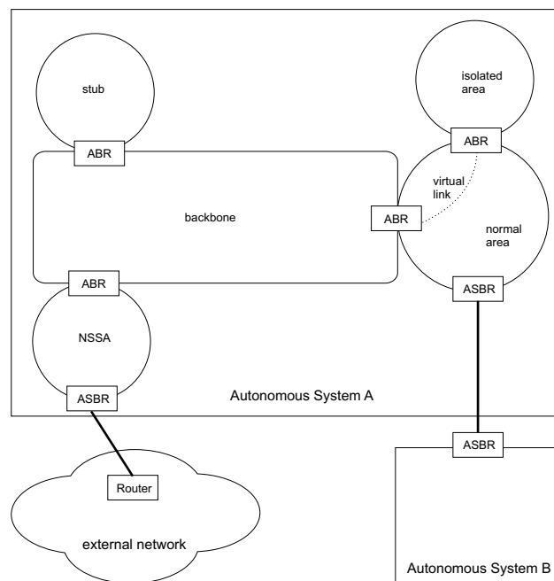
Figure 543: Configuring OSPF
