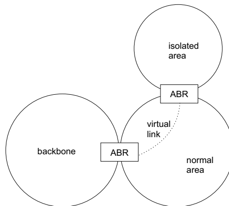
Figure 563: OSPF Virtual Link
