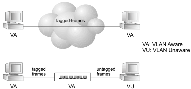
Figure 82: VLAN Compliant and VLAN Non-compliant Devices
