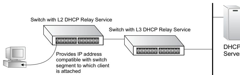
Figure 488: Layer 2 DHCP Relay Service (DHCP server on a separate network segment)
