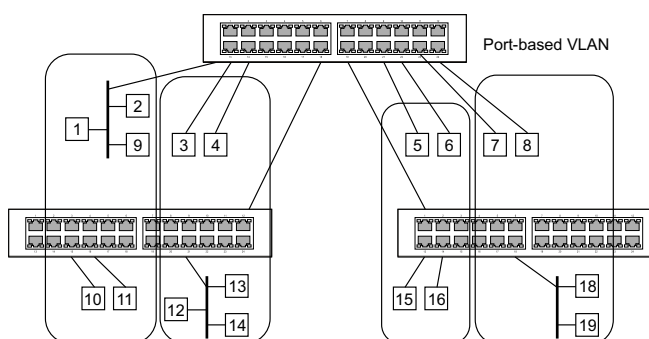
Figure 83: Using GVRP
