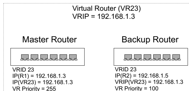
Figure 515: Master Virtual Router with Backup Routers
