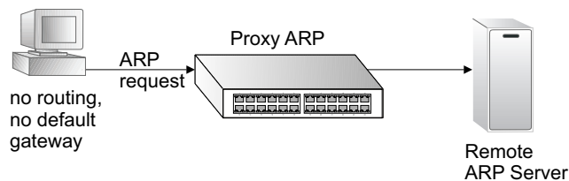
Figure 454: Proxy ARP
