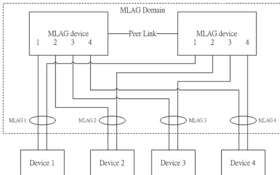
Figure 332: MLAG Domain Topology
