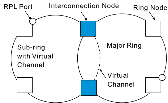
Figure 326: Sub-ring with Virtual Channel
