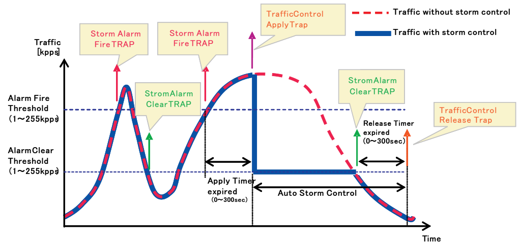
Figure 146: Storm Control by Limiting the Traffic Rate
