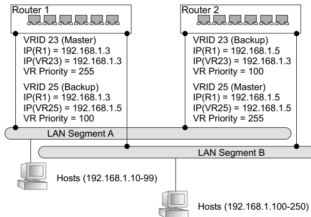
Figure 517: Several Virtual Master Routers Configured for Mutual Backup and Load Sharing
