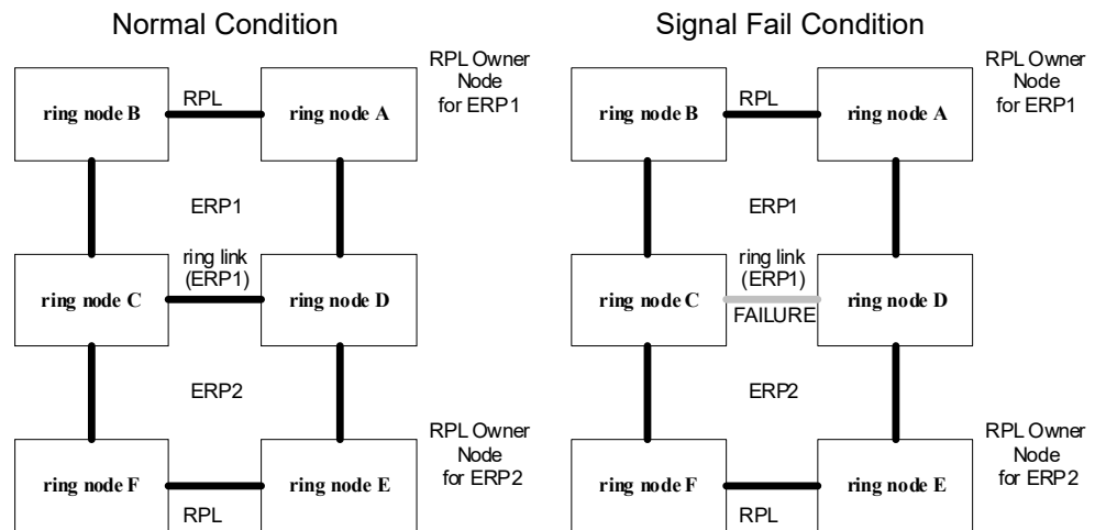
Figure 322: Ring Interconnection Architecture (Multi-ring/Ladder Network)
