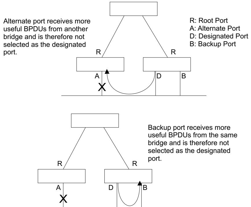
Figure 134: STA Port Roles
