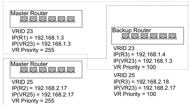
Figure 517: Several Virtual Master Routers Configured for Mutual Backup and Load Sharing
