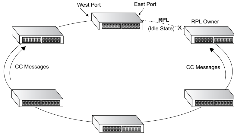
Figure 321: ERPS Ring Components
