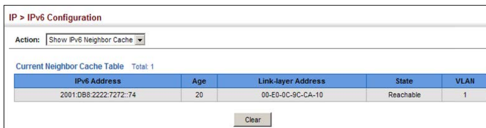
Figure 441: Showing IPv6 Neighbors
