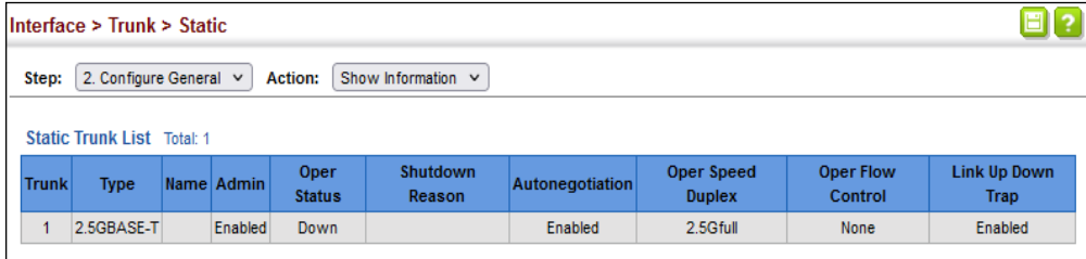
Figure 50: Showing Information for Static Trunks
