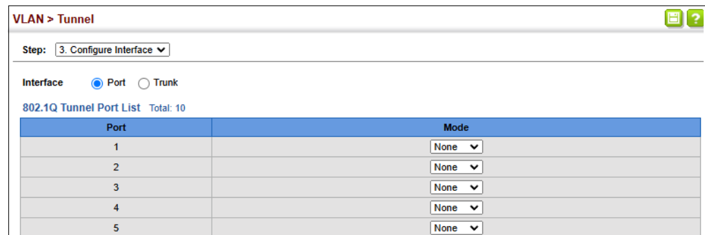
Figure 97: Adding an Interface to a QinQ Tunnel
