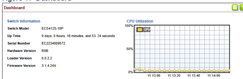
Figure 1: Dashboard
