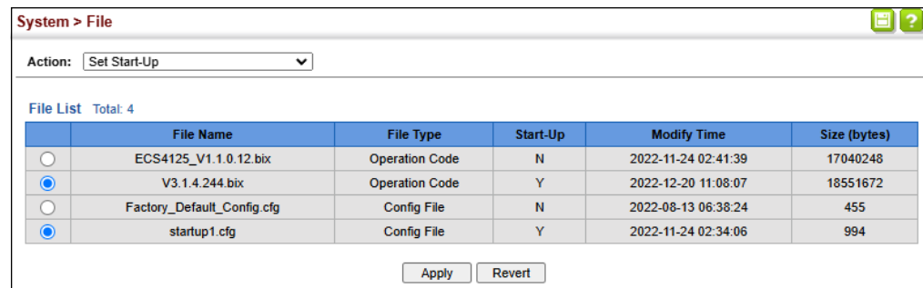
Figure 10: Setting Start-Up Files
