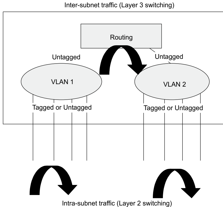
Figure 476: Virtual Interfaces and Layer 3 Routing
