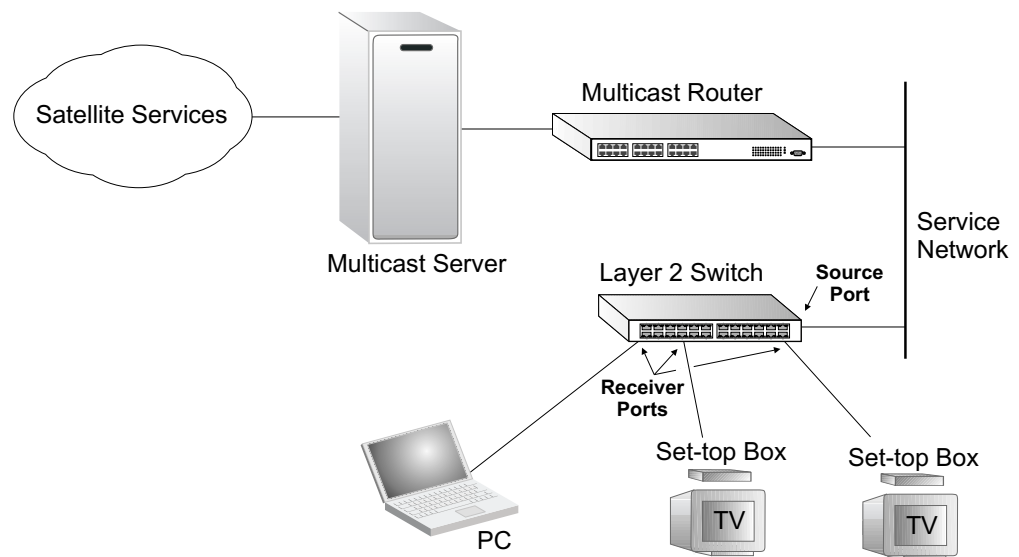
Figure 398: MVR Concept
