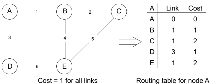
Figure 480: Configuring RIP
