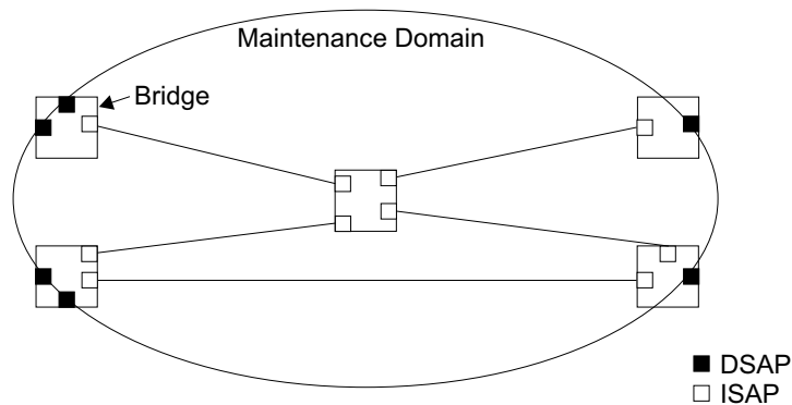
Figure 315: Single CFM Maintenance Domain
