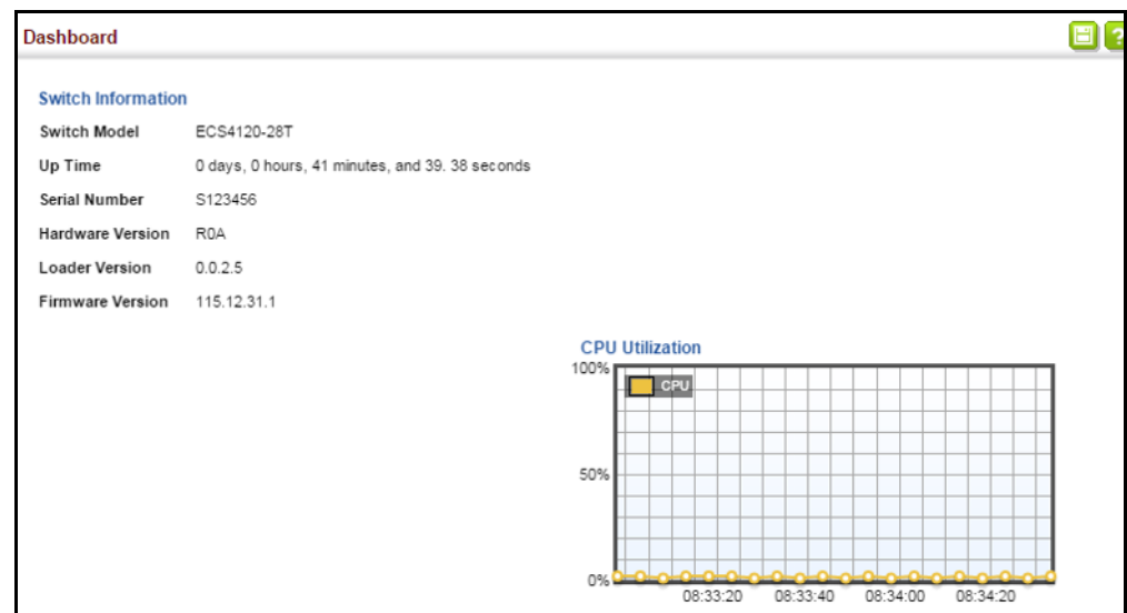
Figure 1: Dashboard
