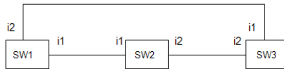
Figure 101: Determining the Root Port
