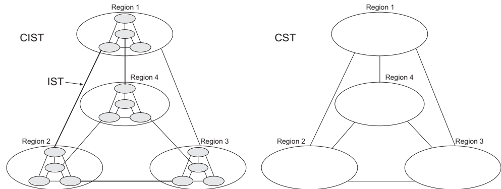
Figure 95: Spanning Tree – Common Internal, Common, Internal
