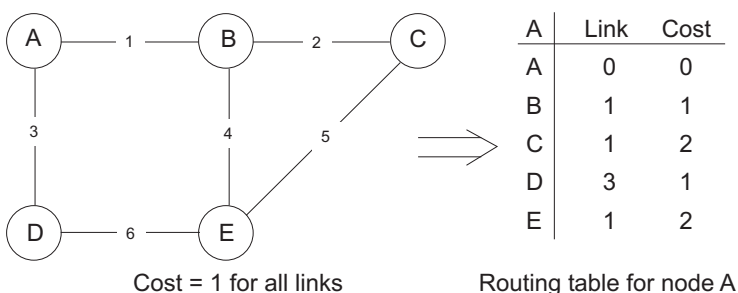
Figure 327: Configuring RIP
