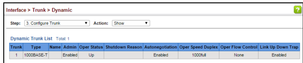
Figure 54: Showing Connection Parameters for Dynamic Trunks
