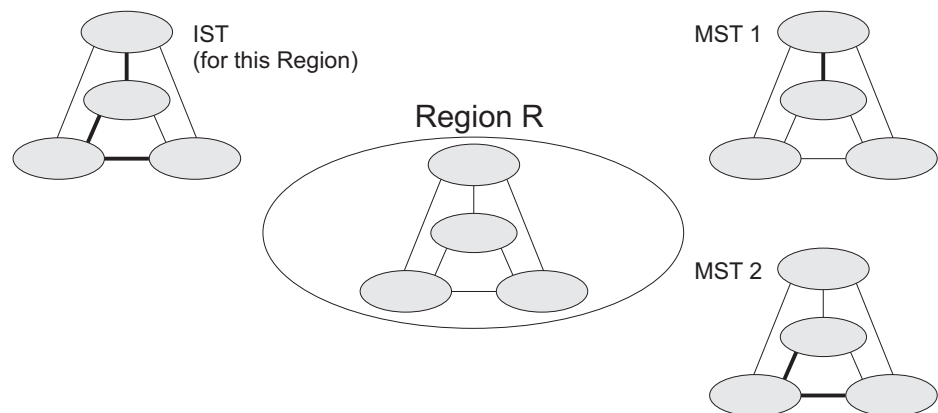
Figure 94: MSTP Region, Internal Spanning Tree, Multiple Spanning Tree
