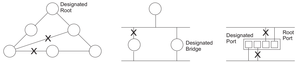
Figure 93: STP Root Ports and Designated Ports
