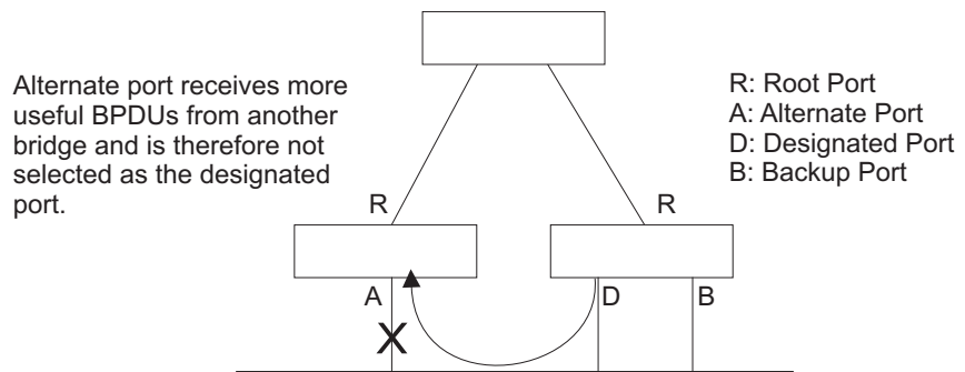
Figure 103: STA Port Roles
