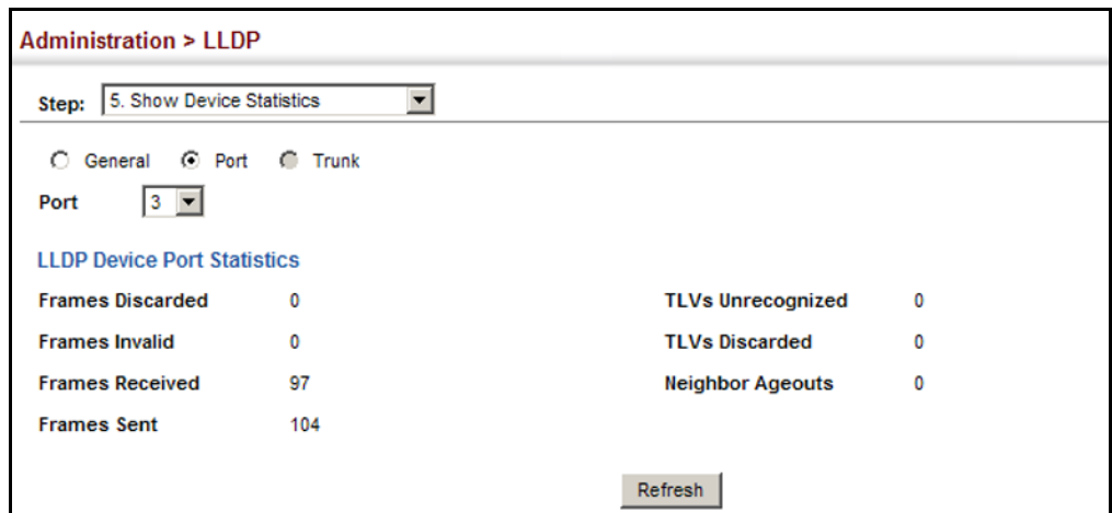
Figure 214: Displaying LLDP Device Statistics (Port)
