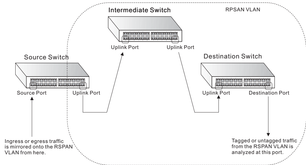
Figure 60: Configuring Remote Port Mirroring
