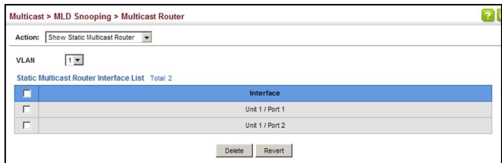
Figure 286: Showing Static Interfaces Attached an IPv6 Multicast Router
