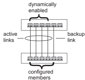
Figure 49: Configuring Dynamic Trunks
