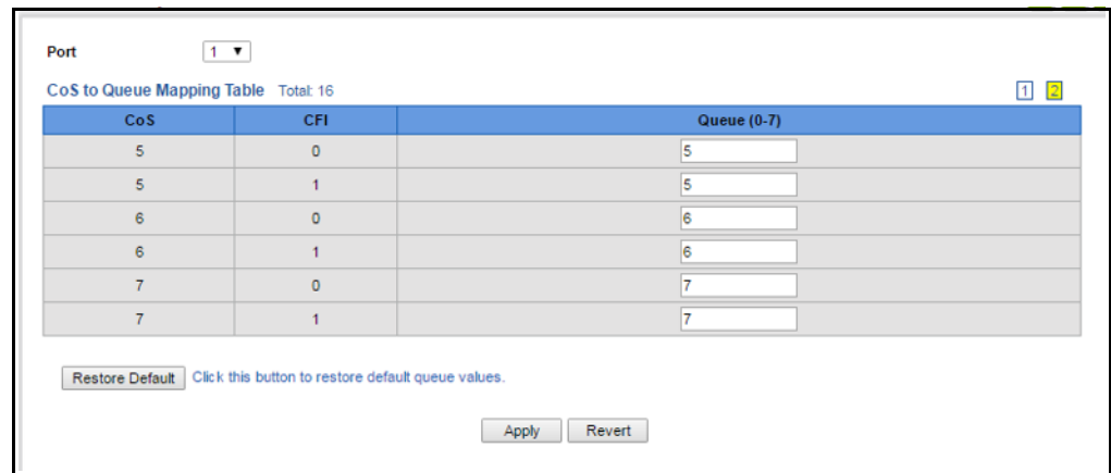
Figure 120: Configuring CoS to Queue Mapping
