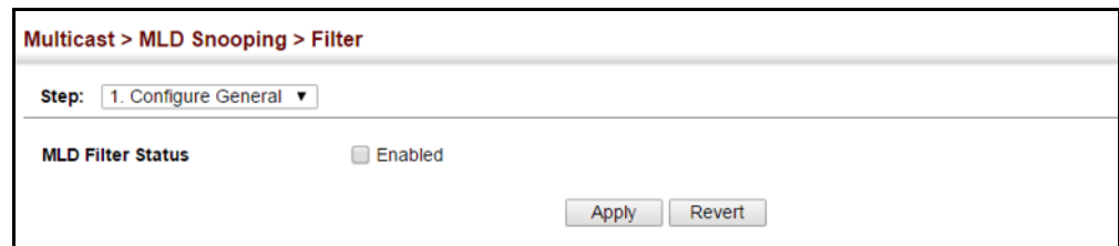
Figure 298: Enabling MLD Filtering and Throttling
