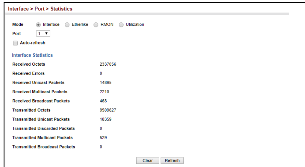
Figure 34: Showing Port Statistics (Table)
