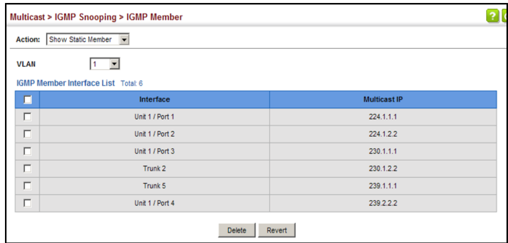
Figure 268: Showing Static Interfaces Assigned to a Multicast Service
