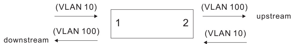
Figure 95: Configuring VLAN Translation
