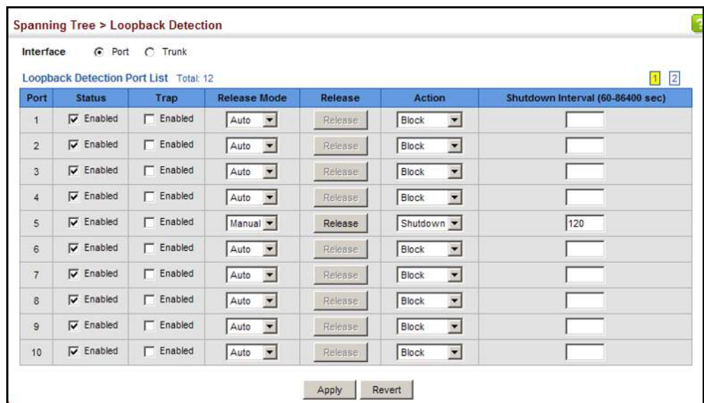
Figure 110: Configuring Port Loopback Detection
