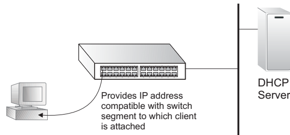
Figure 357: Layer 2 DHCP Relay Service
