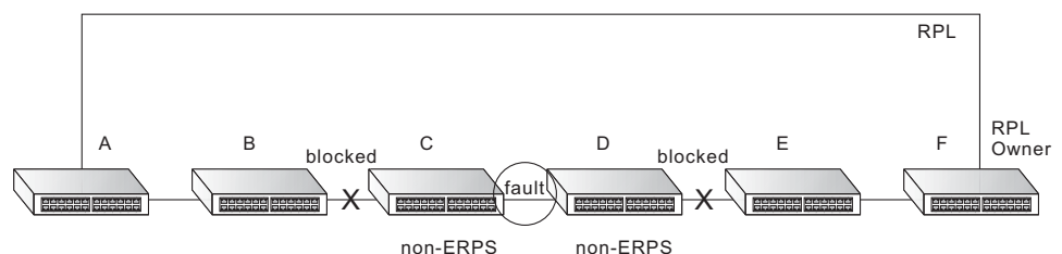
Figure 293: Non-ERPS Device Protection
