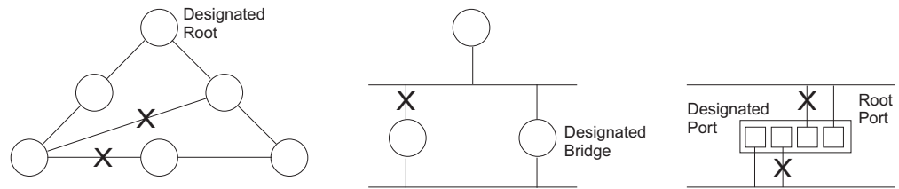
Figure 107: STP Root Ports and Designated Ports
