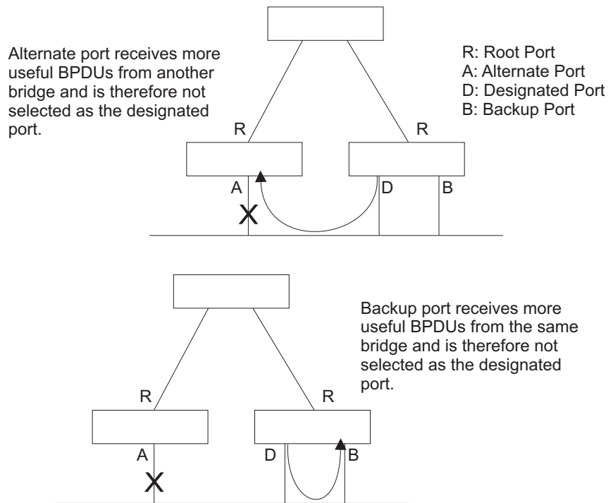
Figure 117: STA Port Roles
