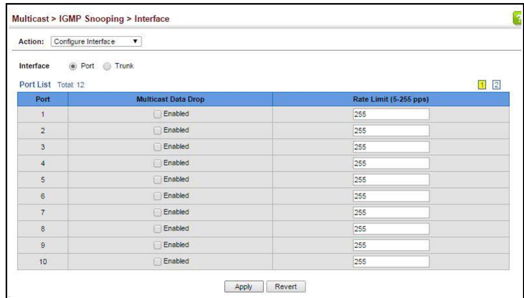
Figure 372: Dropping IGMP Query or Report Packets
