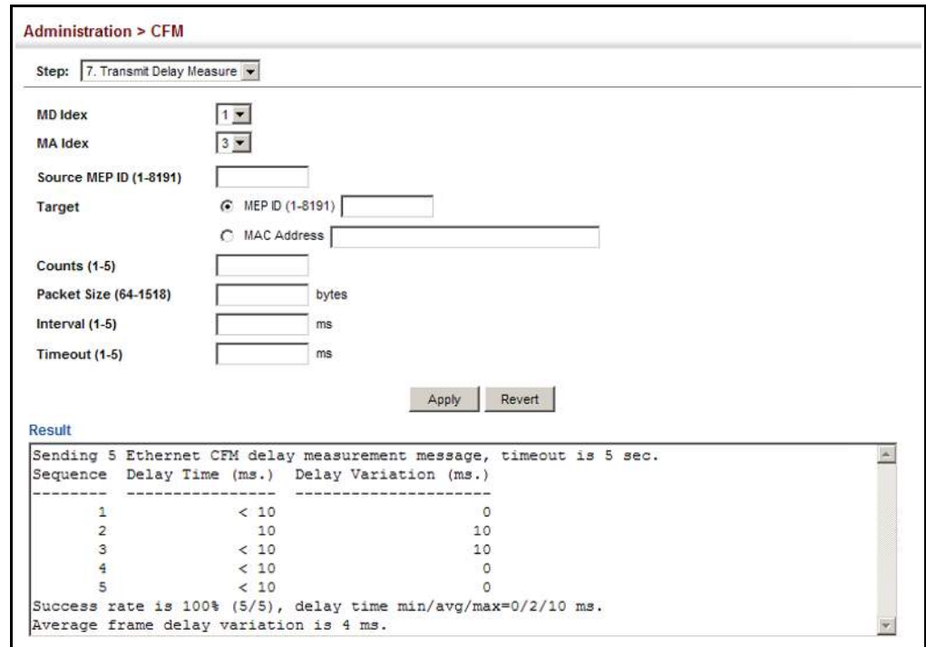
Figure 314: Transmitting Delay-Measure Messages
