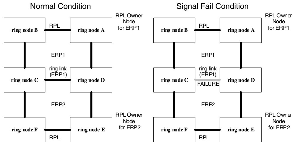
Figure 289: Ring Interconnection Architecture (Multi-ring/Ladder Network)
