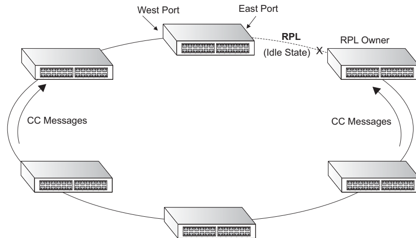
Figure 288: ERPS Ring Components
