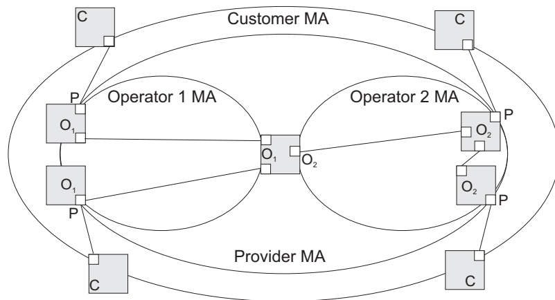
Figure 299: Multiple CFM Maintenance Domains
