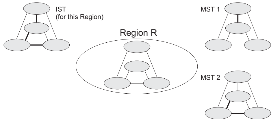
Figure 108: MSTP Region, Internal Spanning Tree, Multiple Spanning Tree
