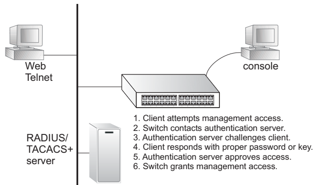
Figure 160: Authentication Server Operation
