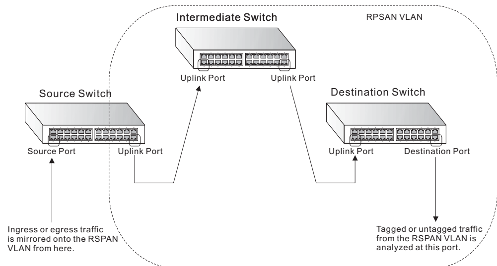
Figure 31: Configuring Remote Port Mirroring
