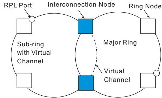
Figure 291: Sub-ring with Virtual Channel
