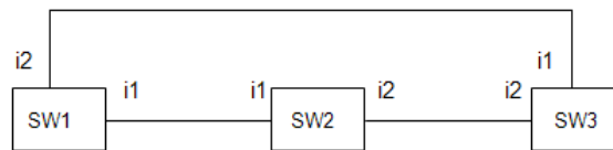
Figure 115: Determining the Root Port
