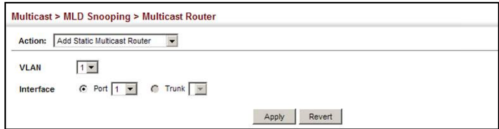
Figure 385: Configuring a Static Interface for an IPv6 Multicast Router
