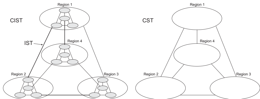
Figure 109: Spanning Tree – Common Internal, Common, Internal
