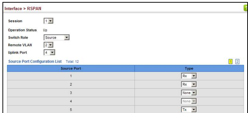
Figure 32: Configuring Remote Port Mirroring (Source)
