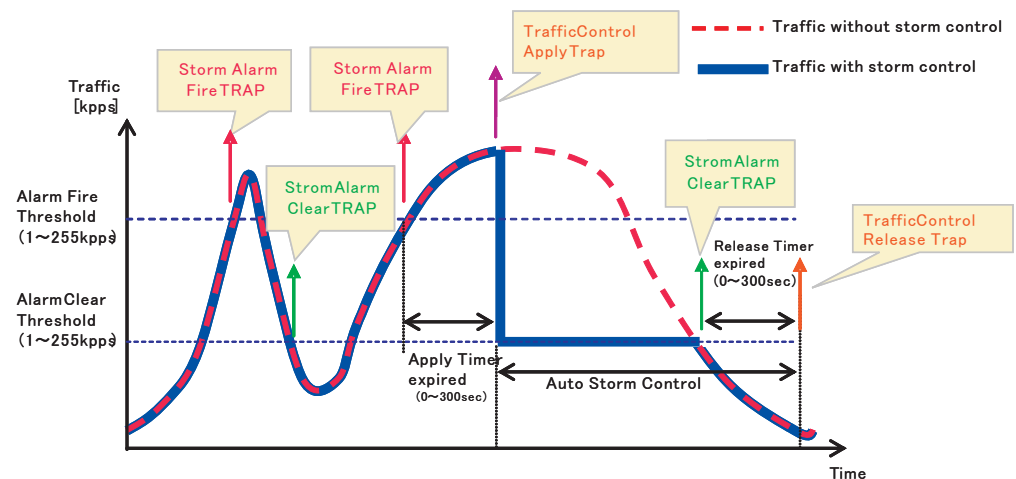
Figure 129: Storm Control by Limiting the Traffic Rate
