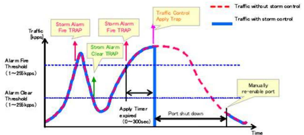
Figure 130: Storm Control by Shutting Down a Port
