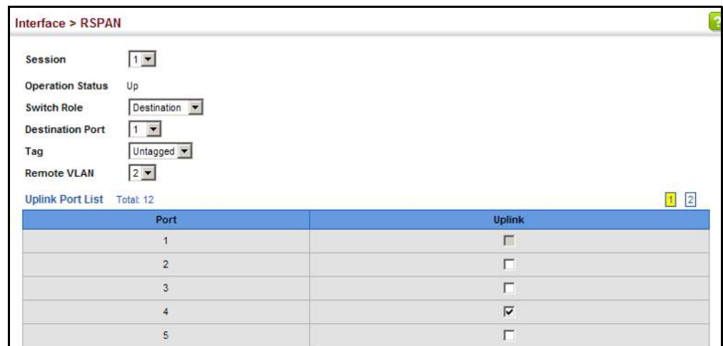
Figure 34: Configuring Remote Port Mirroring (Destination)
