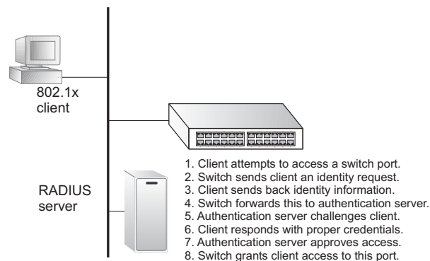
Figure 218: Configuring Port Authentication
