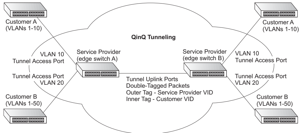
Figure 80: QinQ Operational Concept
