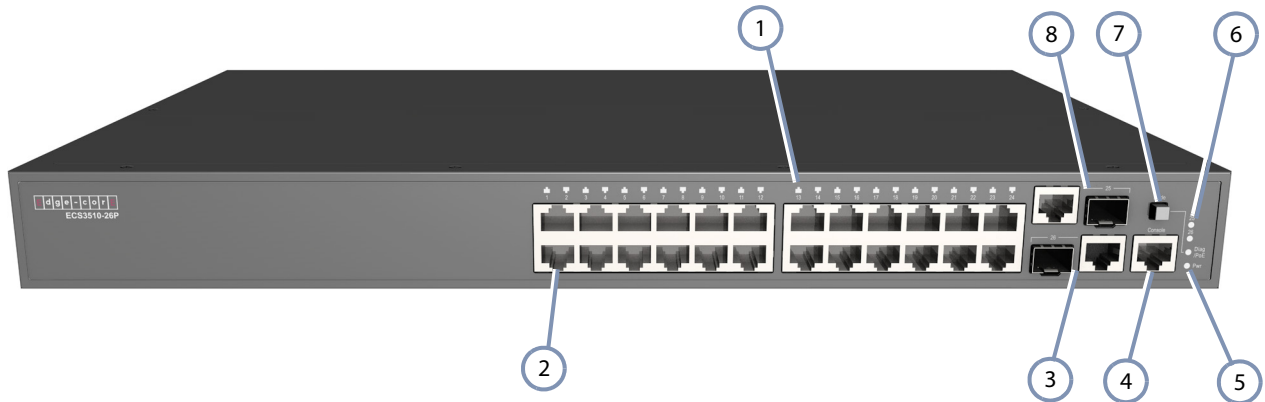
Figure 1: Front Panel ECS3510-26P
