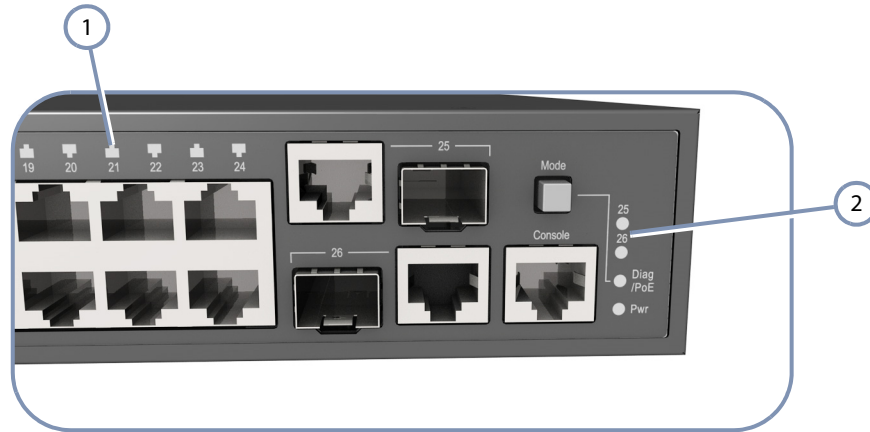
Figure 15: Port Status LEDs
