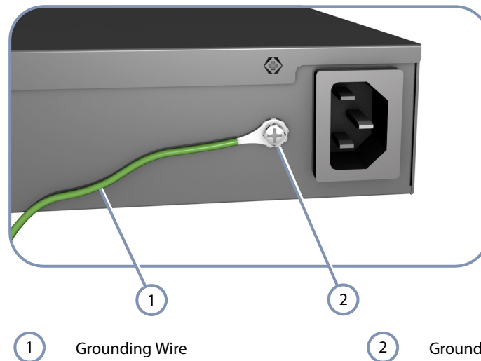
Figure 13: Grounding Terminal
