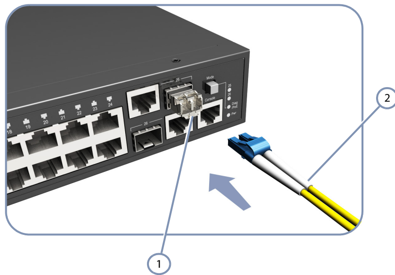
Figure 7: Making a Connection to an SFP Port
