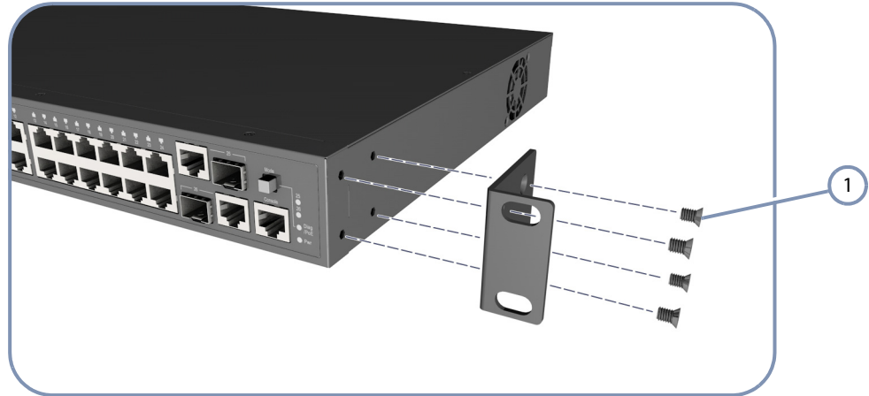
Figure 8: Attaching the Brackets
