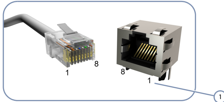
1 RJ-45 Pin Numbers
