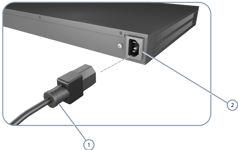
Figure 4: Connecting AC Power
